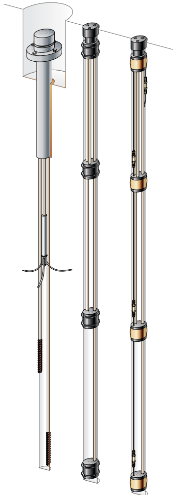
Model A-3, A-4 and A-5 Multiple Point Extensometers (left to right).
