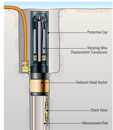
Flangeless type head assembly.
