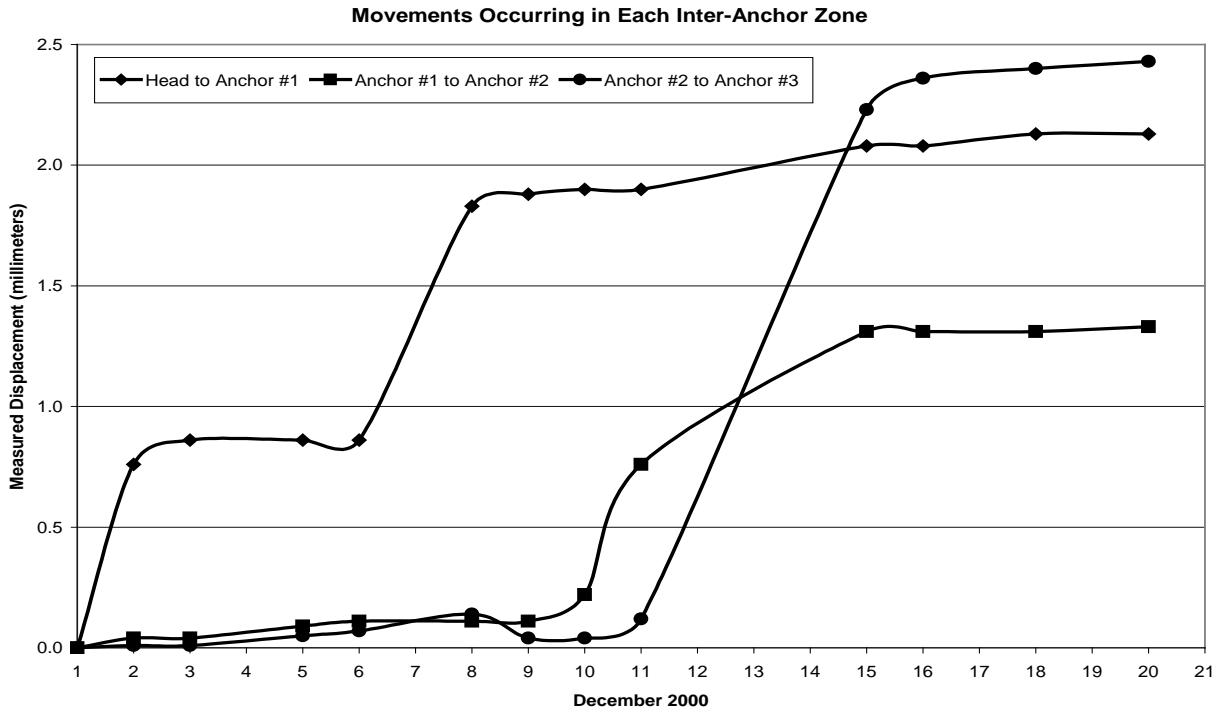
Figure 5 Movements Occurring in Each Inter-Anchor Zone
