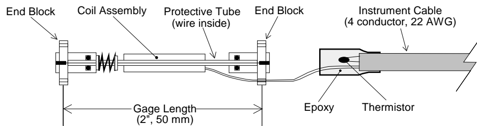
Figure 2 - Model VCE-4202 Vibrating Wire Strain Gage
