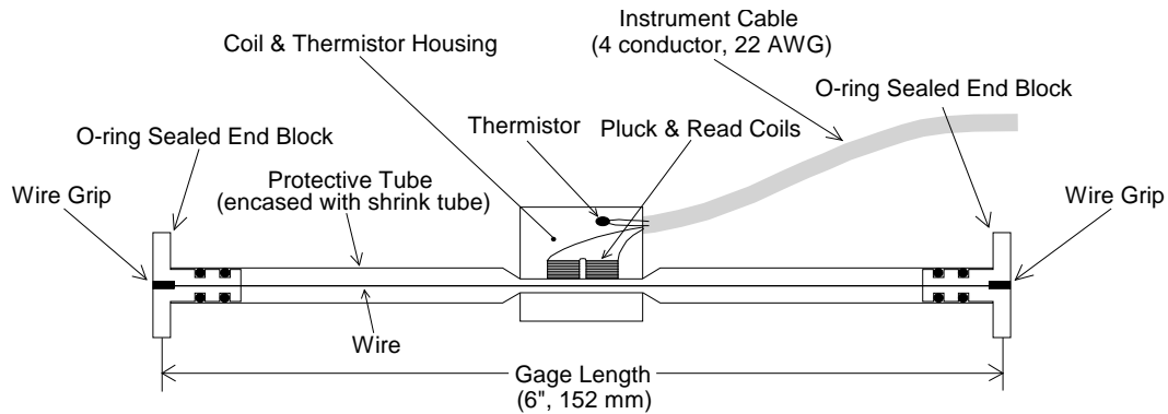
Figure 1 - Model VCE-4200 Vibrating Wire Strain Gage
