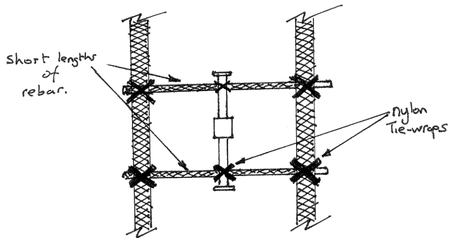
Figure 4B - Alternative Method for attaching VCE 4200 strain gages to rebar.
