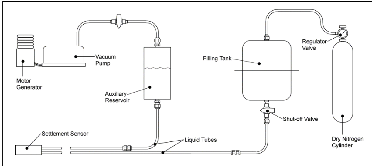
Figure 4. Flushing Apparatus
