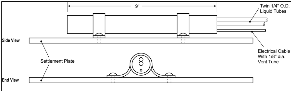
Figure 2. Sensor details.
