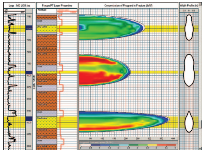
Fracpro can display logs, layer information and geometry with the integrated fracture picture.
